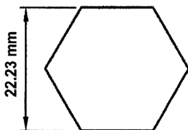
7/8" x 20' MF
