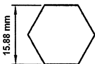
5/8" x 20' MF
