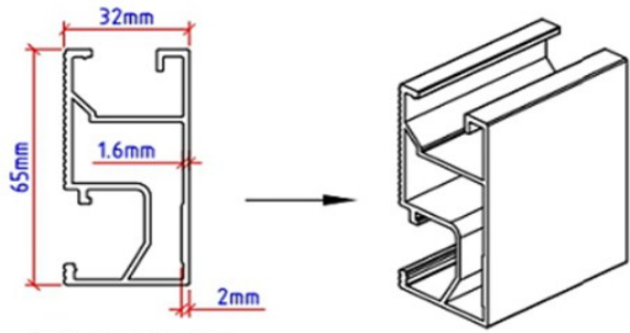
MAIN FRAME LK5275 Scale 1:2 Length : 6.1 M Finishing : N.A
