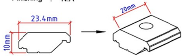
SCREW NUT LK5277 Scale 1:1 Length : 20 mm Finishing : M.F
