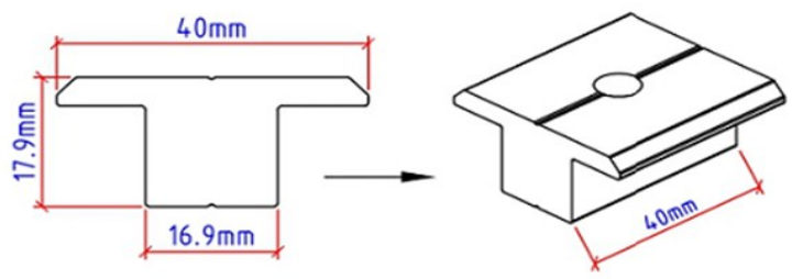
CENTRE T BRACKET LK5278 Scale 1:1 Length : 40 mm Finishing : M.F
