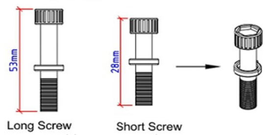
Stainless Steel 304 M8 Short Screw With Spring Washer
