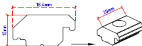
SCREW NUT LK6474
