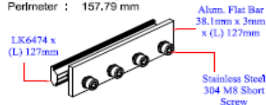
Extension Joint - Type A
