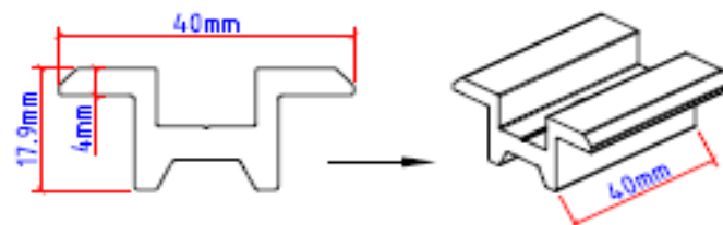
CENTRE T BRACKET LK6472
