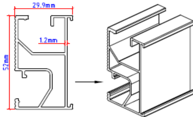
MAIN FRAME LK6471
