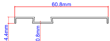
SJ259 (Skirting)
