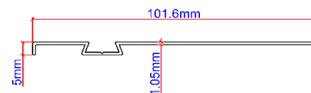
FF806B (Skirting)
