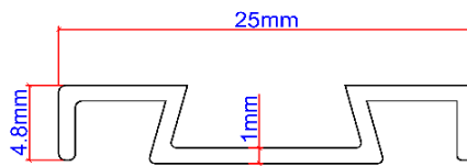
SJ258 (Trimming)
