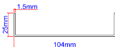
CK4448 (U-Channel)
